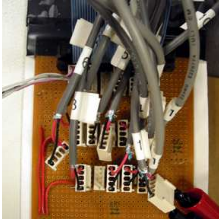
Figure 2-12 Reconfigurable board for biasing the laser
