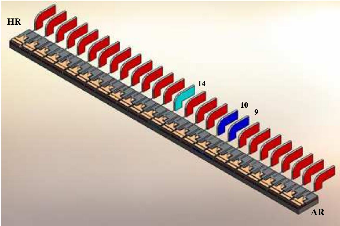
Figure 3-22 Double interval configuration for the generation of the sixth harmonic
