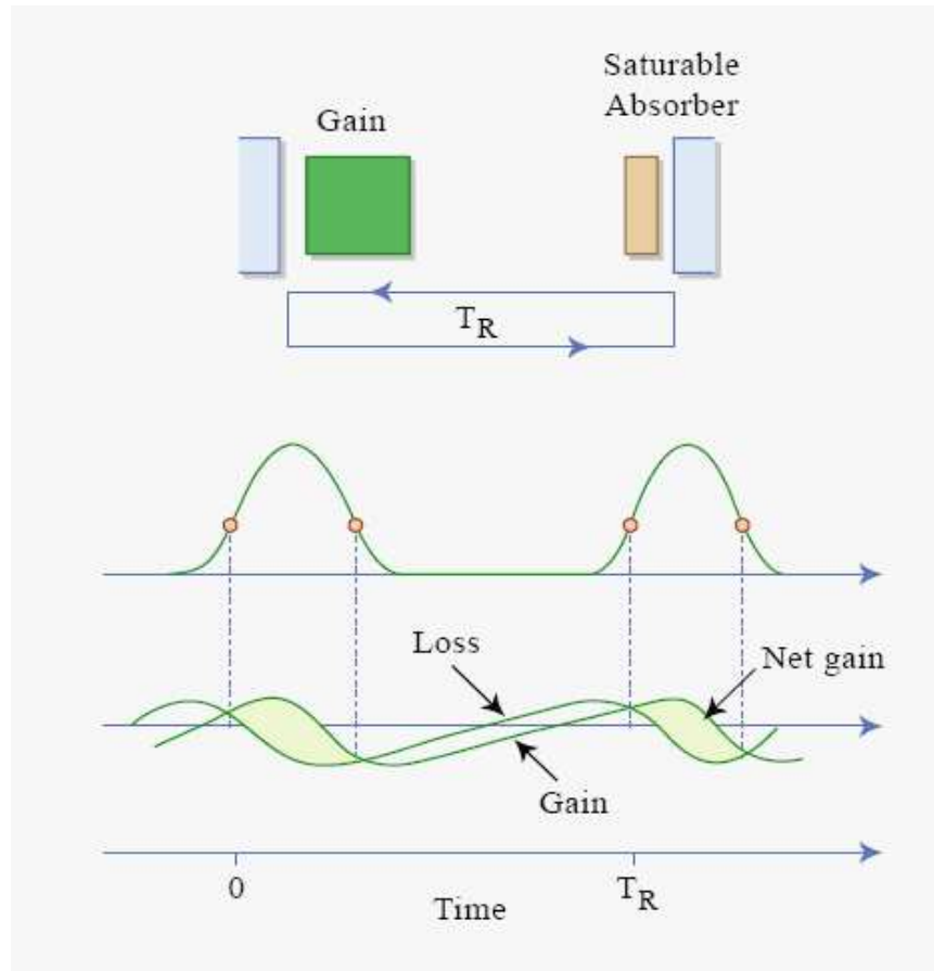
Figure 1-1 The creation of pulses using the internal gain and loss of a laser [8]
