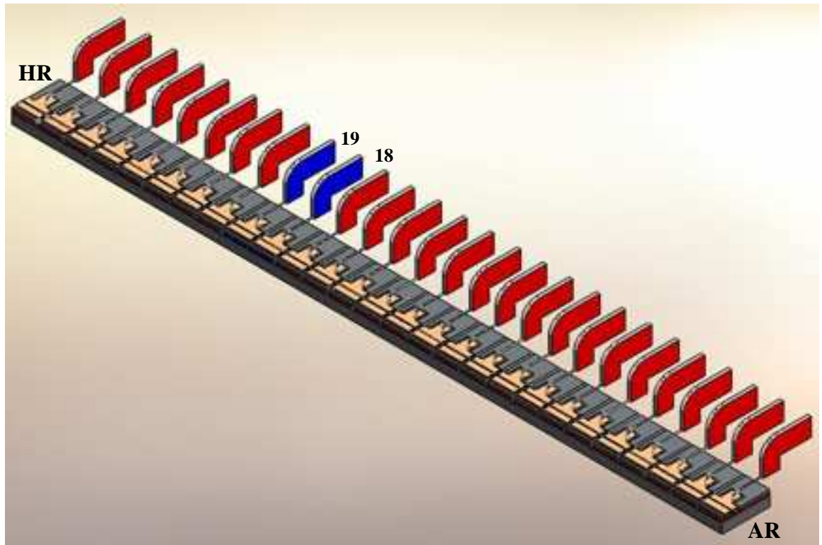
Figure 3-12 Configuration for the generation of the third harmonic
