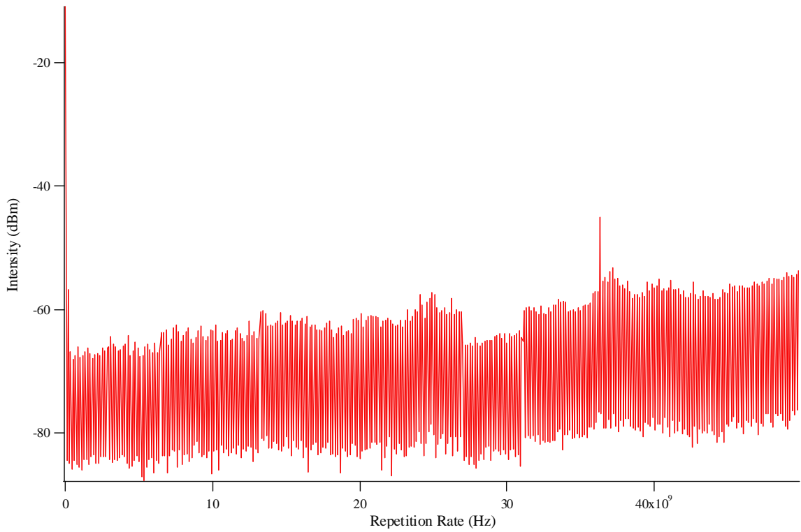
Figure 3-23 50 GHz Span of repetition rate while configured for sixth harmonic generation
