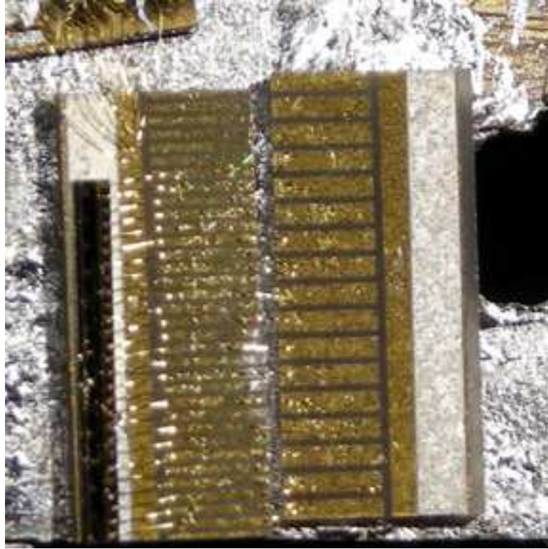
Figure 2-8 The 250- \mu\text{m} and 500- \mu\text{m} contact-pad AlN substrates
