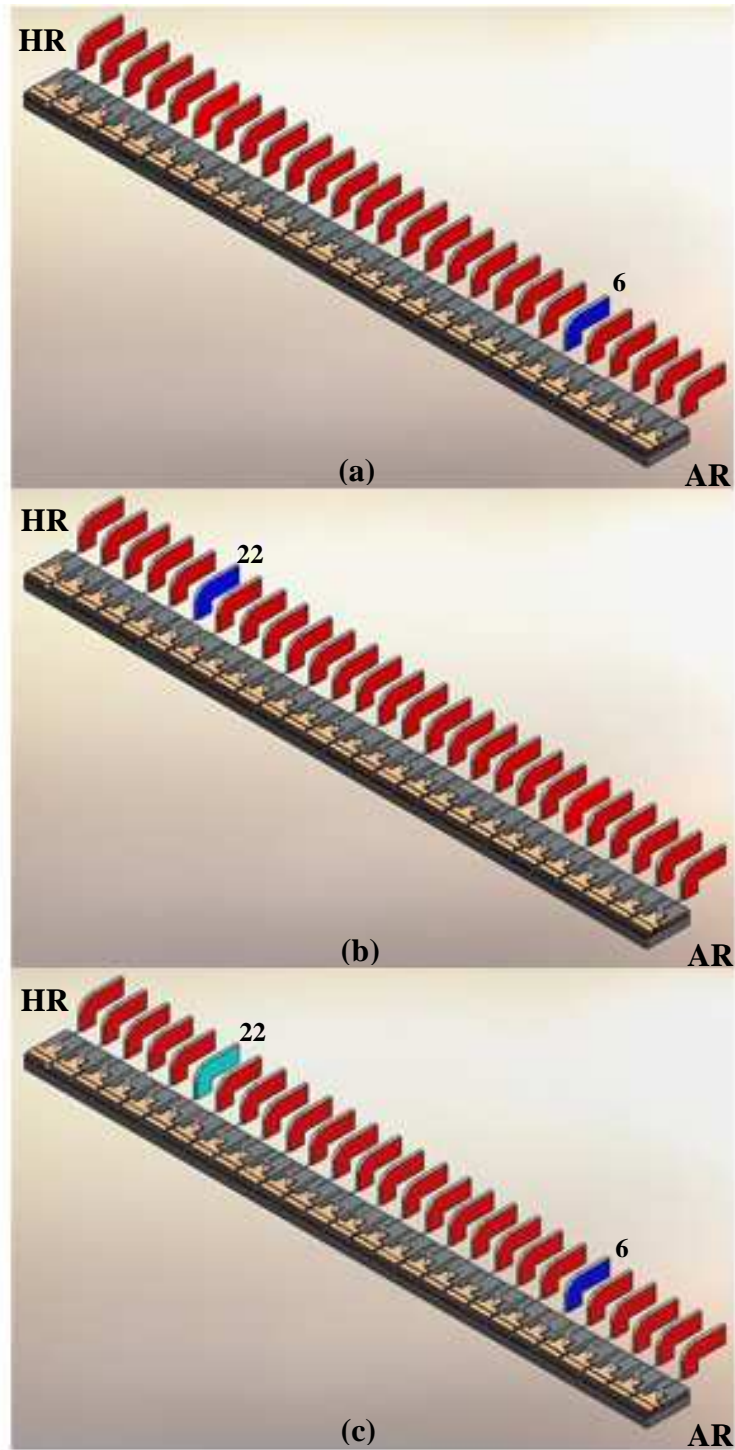
Figure 3-16 Possible configuration for the generation of the fifth harmonic. (a) Using only section 6, (b) using only section 22, and (c) using section 6 and 22
