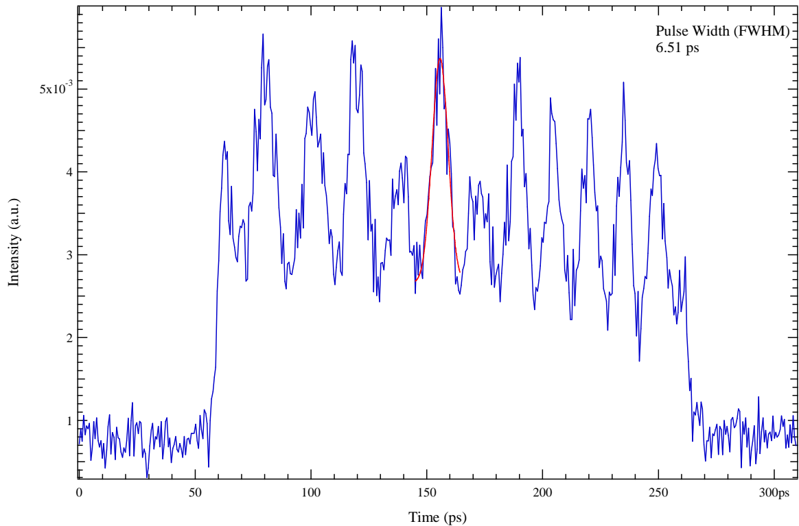
Figure 3-29 Pulse width associated with the tenth harmonic repetition rate
