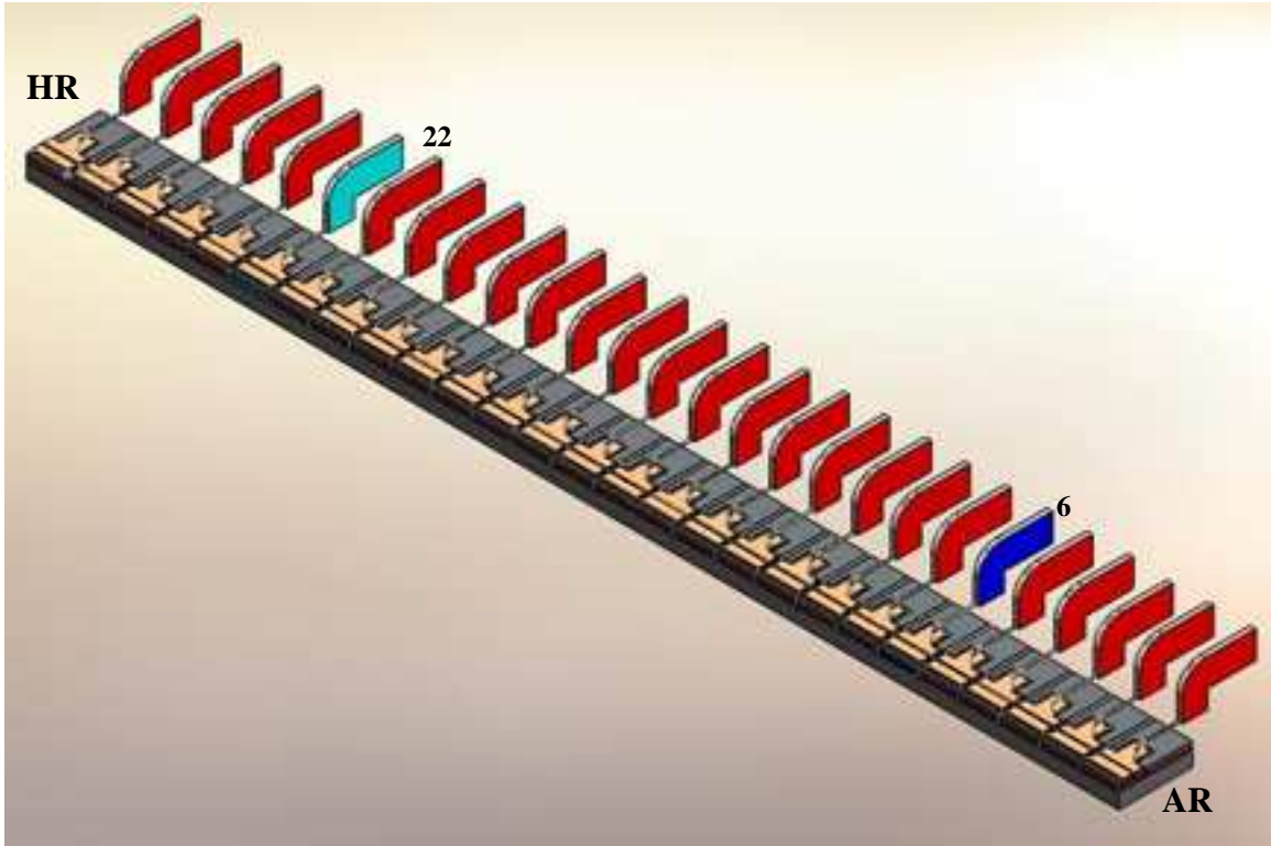
Figure 3-17 Configuration for the generation of the fifth harmonic
