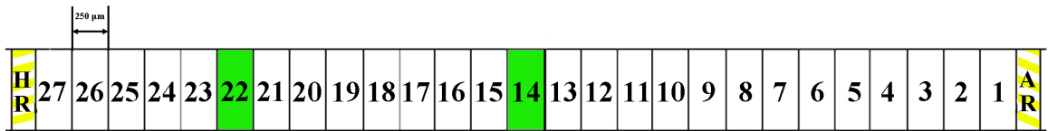
Figure 2-2 Laser anti-nodes for creation of tenth harmonic
