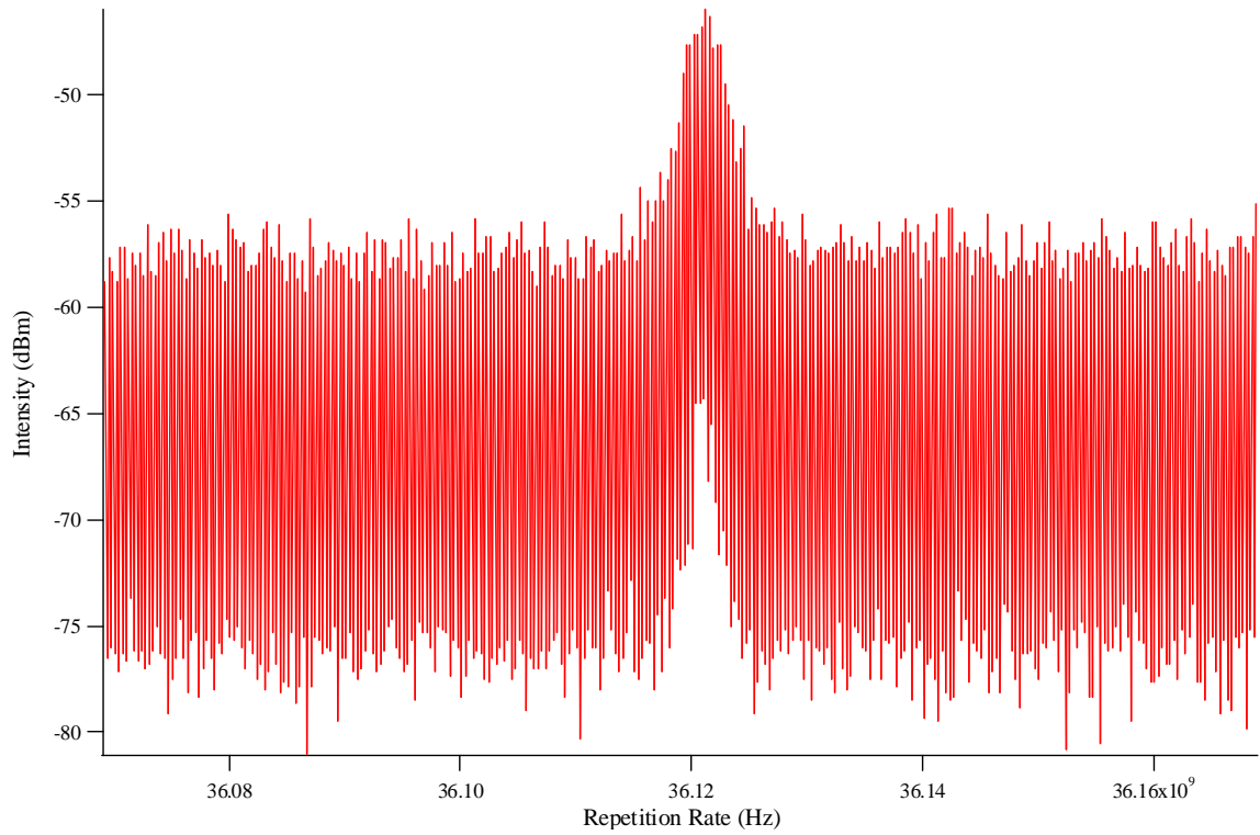
Figure 3-24 100 MHz span of the sixth harmonic repetition rate
