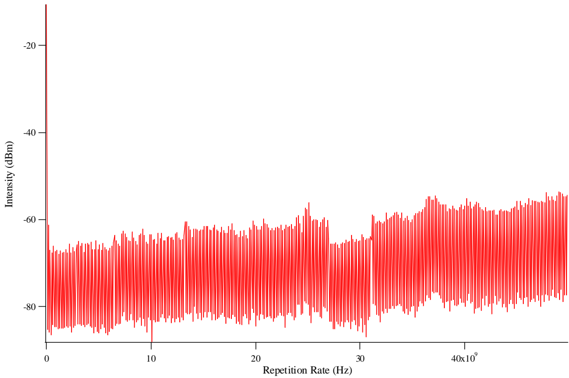
Figure 3-28 50 GHz span of repetition rate while configured for tenth harmonic generation
