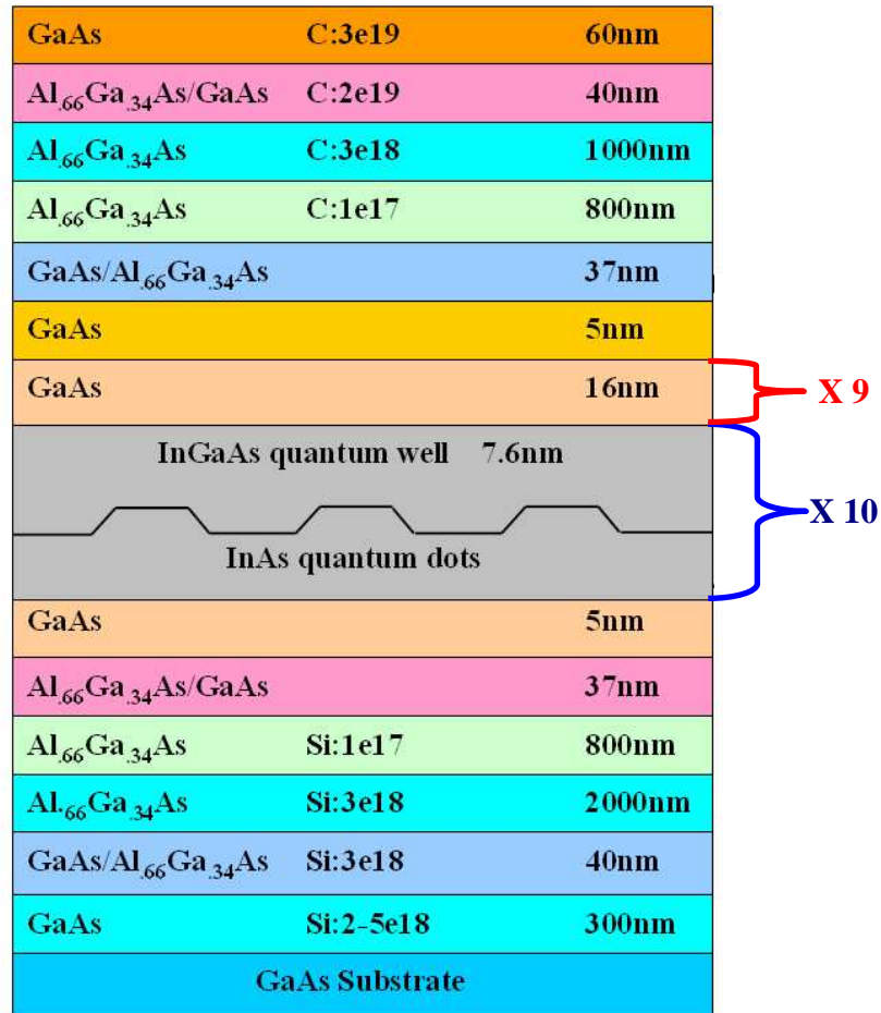
Figure 2-5 Zia Wafer 1023 growth structure
