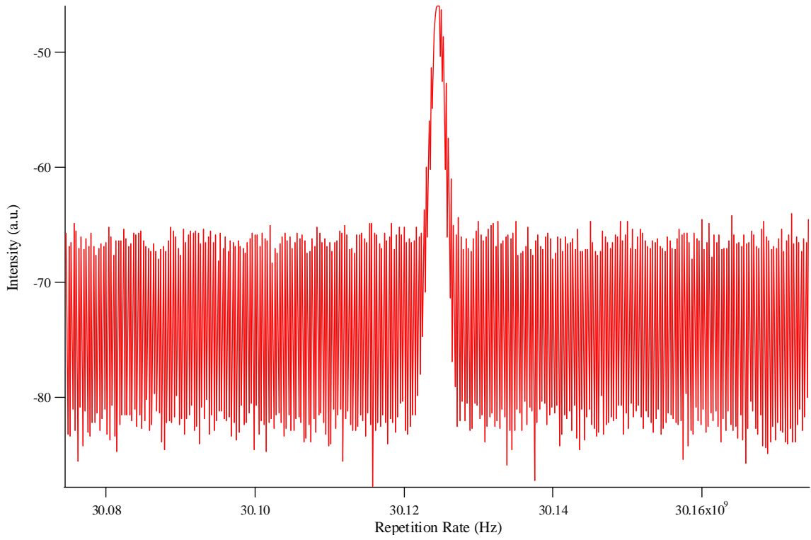
Figure 3-19 100 MHz span of the fifth harmonic repetition rate
