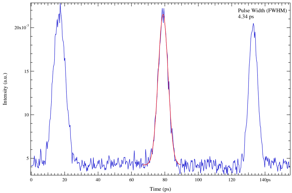
Figure 3-15 Pulse width associated with the third harmonic repetition rate
