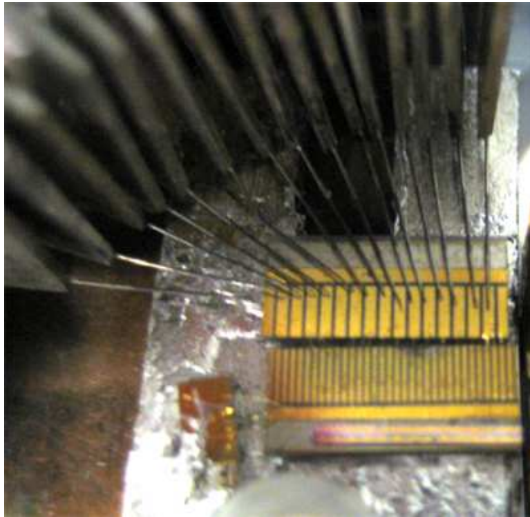
Figure 2-11 Probe card connected to device
