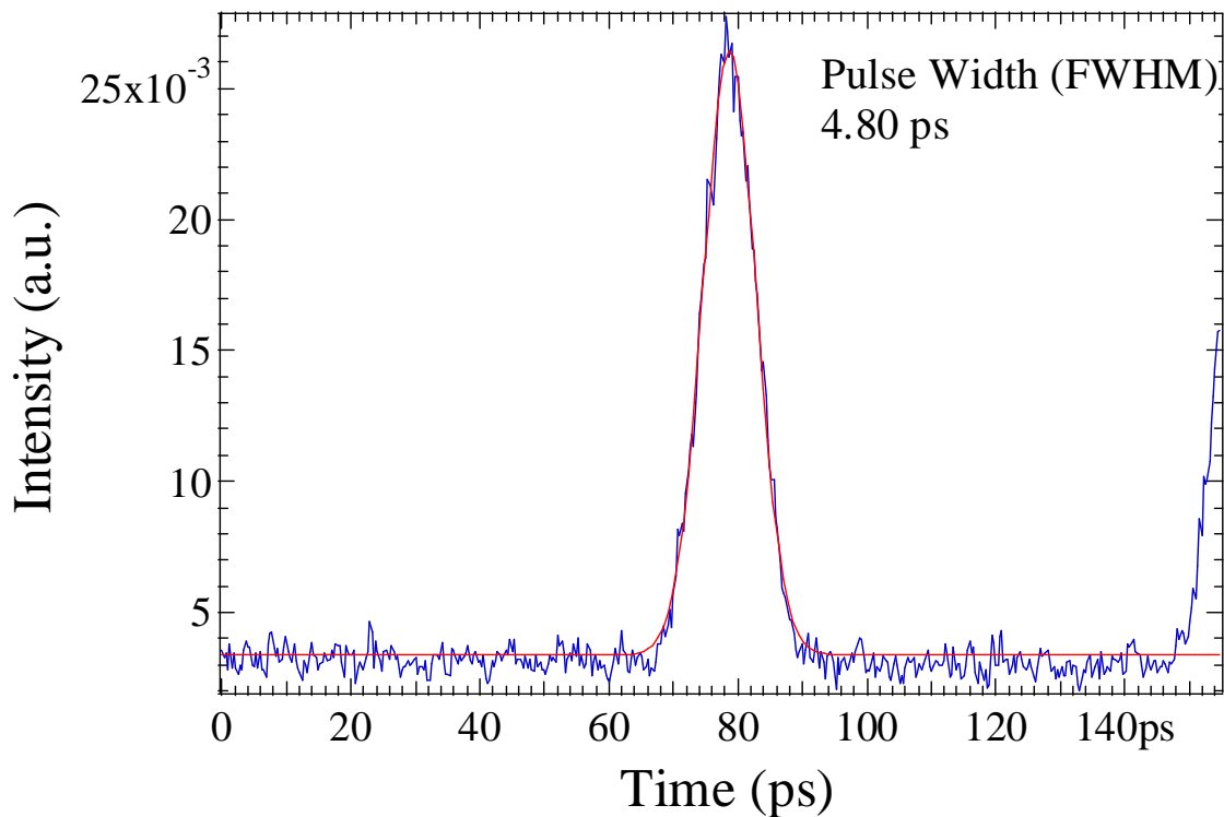
Figure 3-6 Pulse width associated with the second harmonic repetition rate for when three sections of saturable absorber is used
