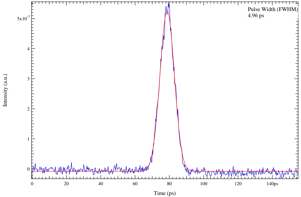
Figure 3-4 Pulse width associated with the fundamental harmonic repetition rate
