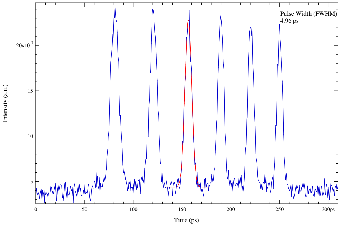
Figure 3-20 Pulse width associated with the fifth harmonic repetition rate
