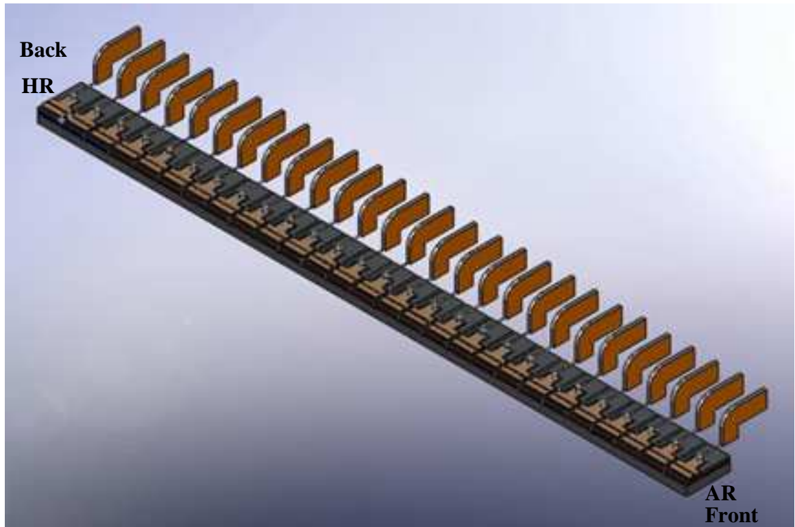
Figure 2-7 Segmented device
