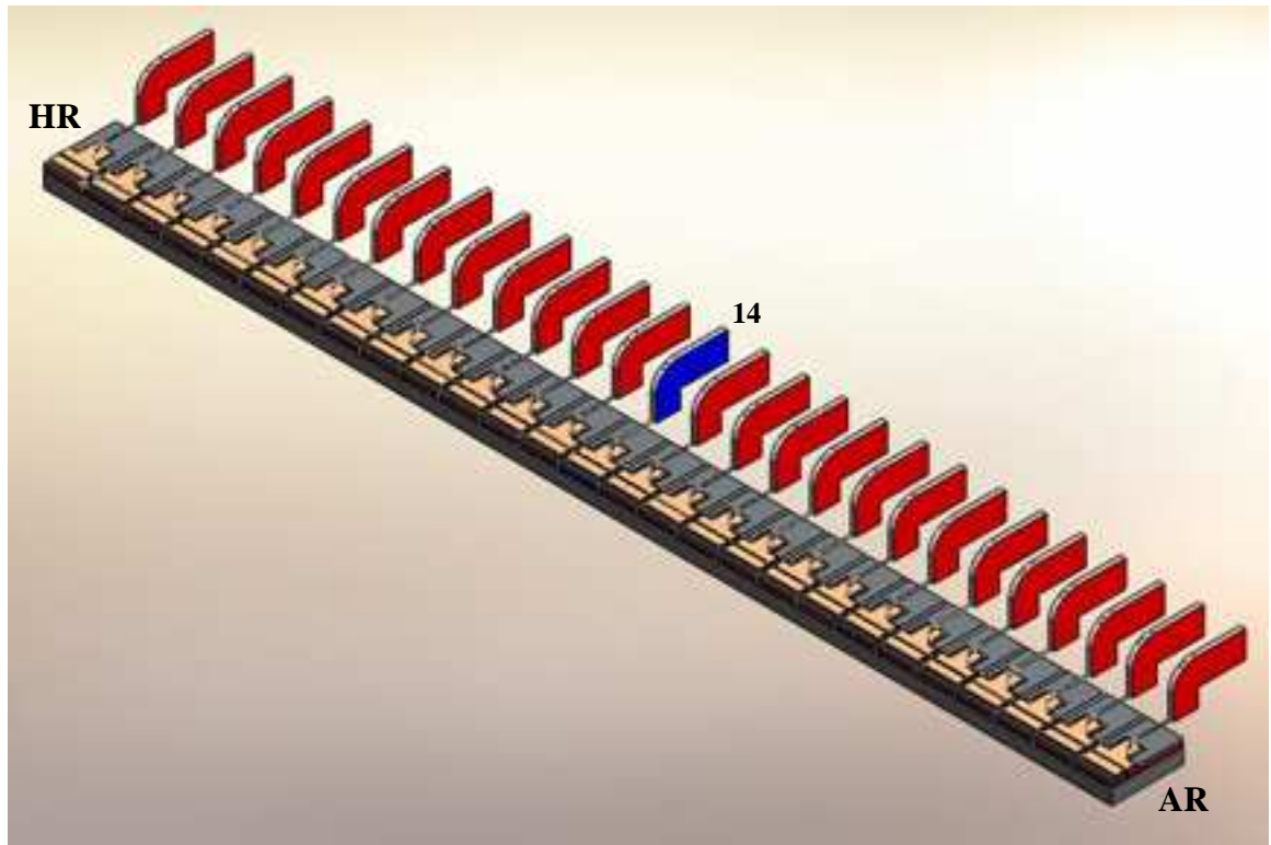
Figure 3-7 Configuration for the generation of the second harmonic
