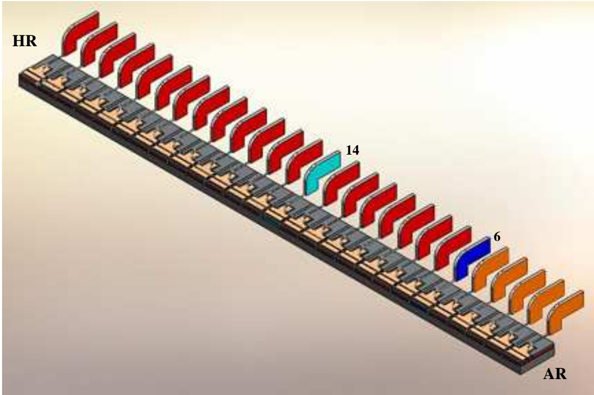
Figure 3-27 Double interval configuration for the generation of the tenth harmonic
