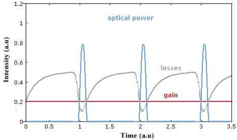
Figure 1-4 An example of a passively mode-locked laser with a slow saturable absorber [12]
