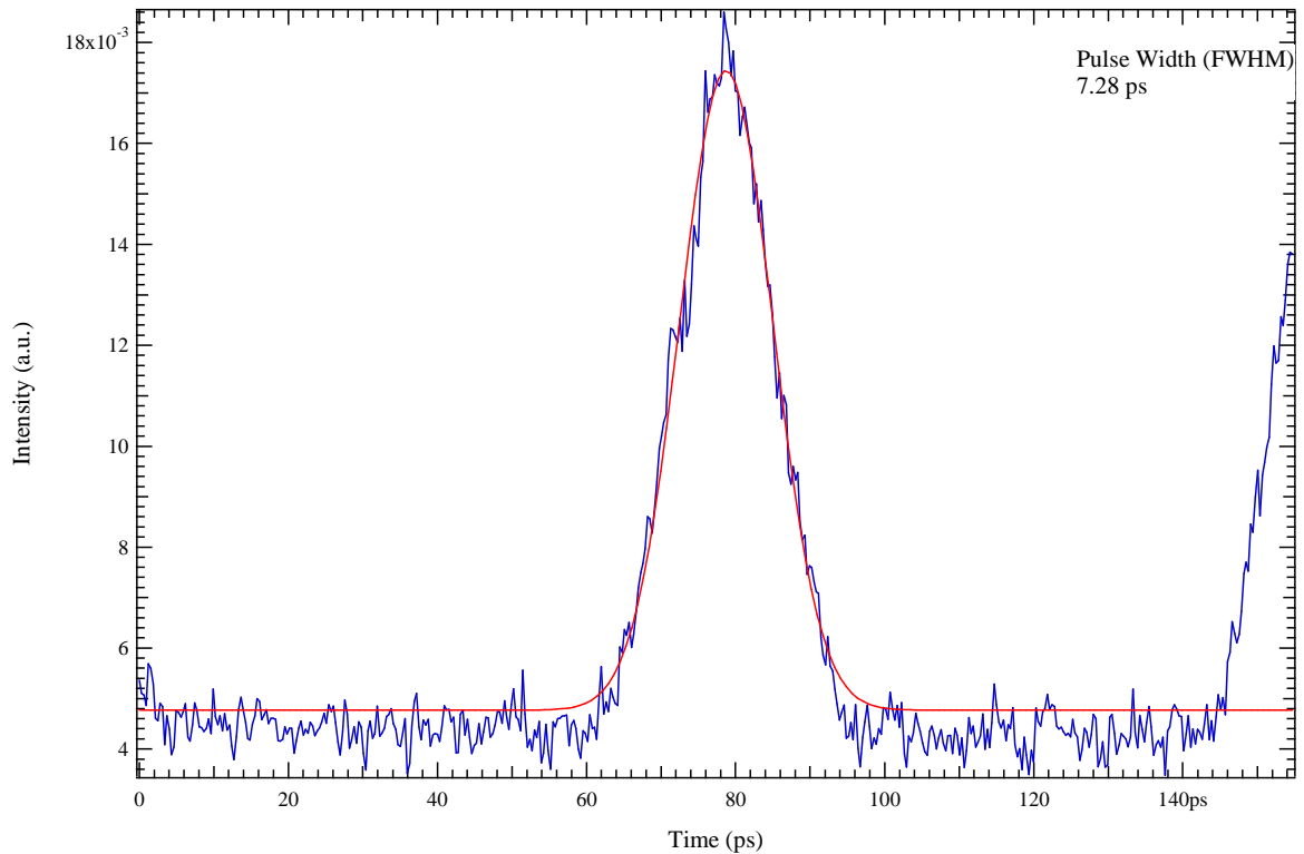
Figure 3-10 Pulse width associated with the second harmonic repetition rate
