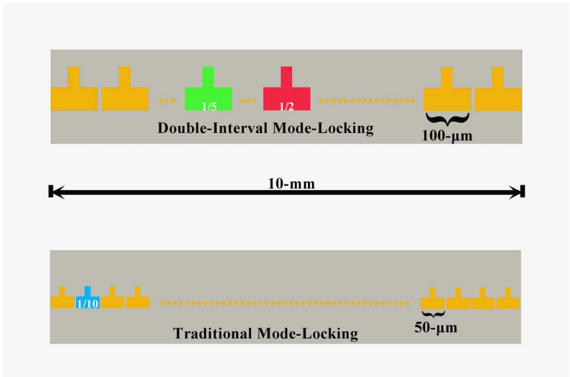
Figure 1-7 Comparison between device segmentation for double-interval mode-locking and traditional mode-locking for the 10 th harmonic of a laser diode
