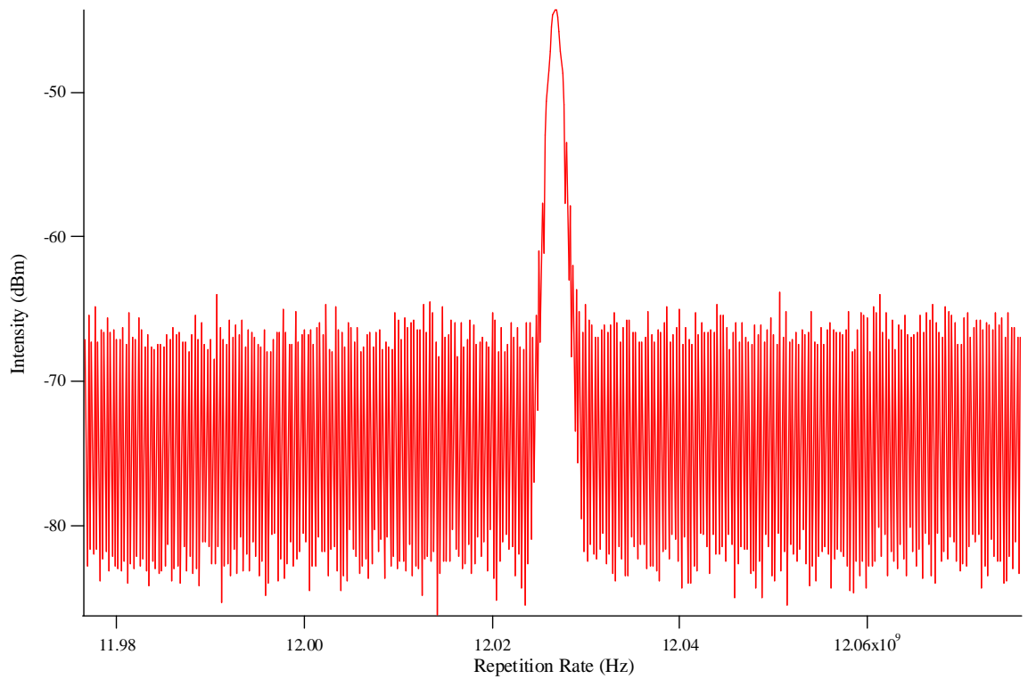
Figure 3-9 100 MHz span of the second harmonic repetition rate
