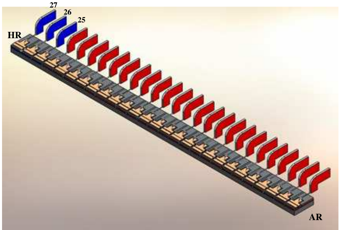
Figure 3-1 Configuration for the generation of the fundamental harmonic
