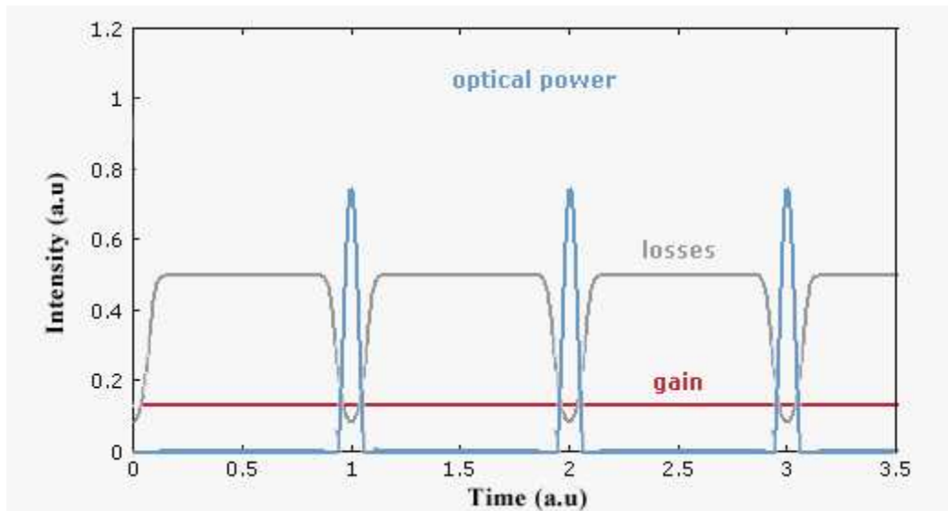
Figure 1-5 An example of a passively mode-locked laser with a fast saturable absorber [12]
