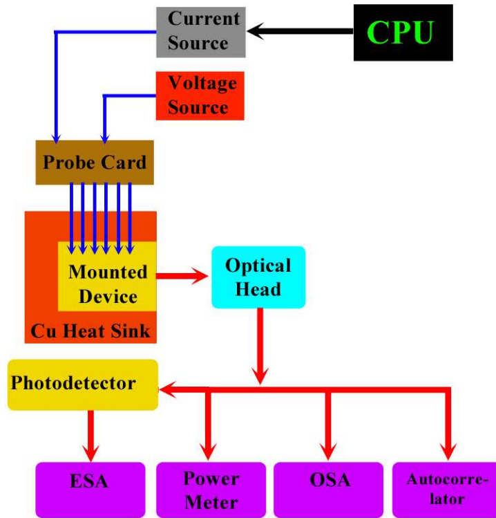
Figure 2-13 Complete system schematic
