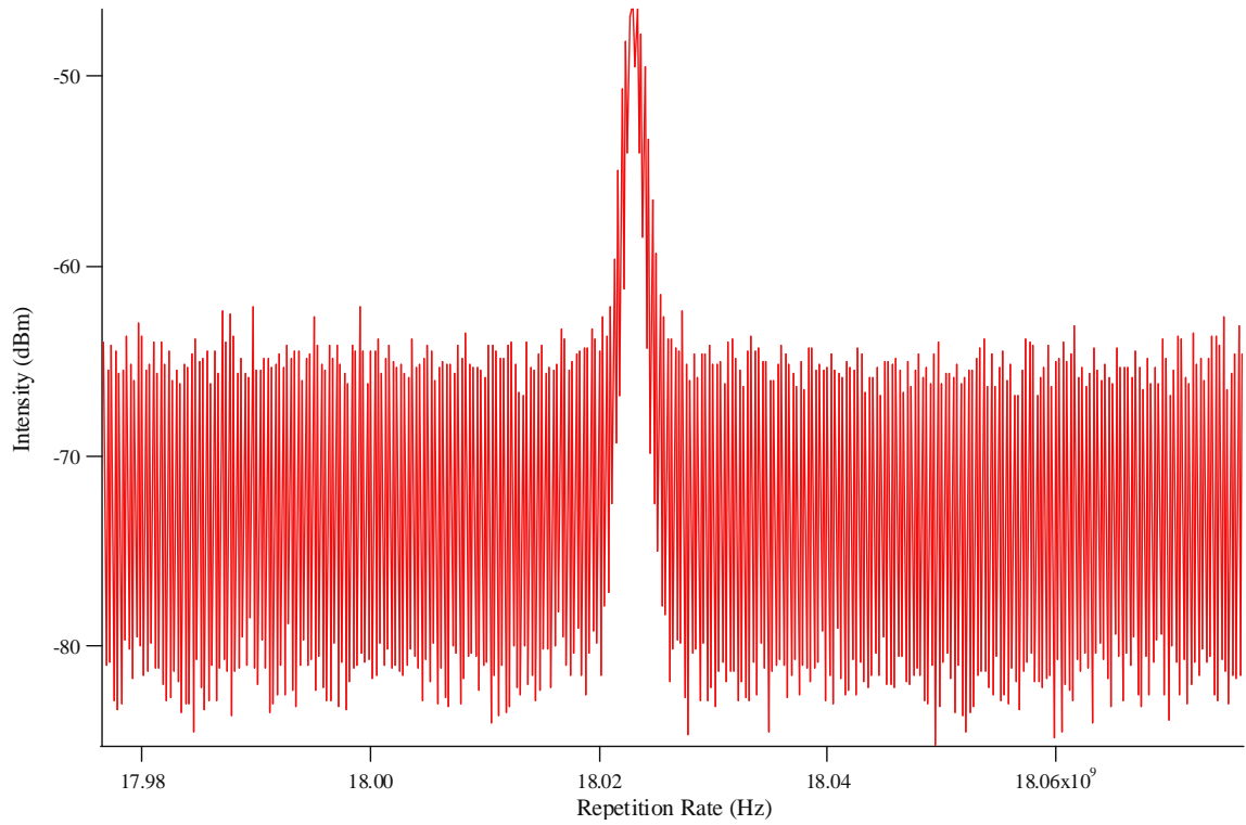
Figure 3-14 100 MHz span of the third harmonic repetition rate
