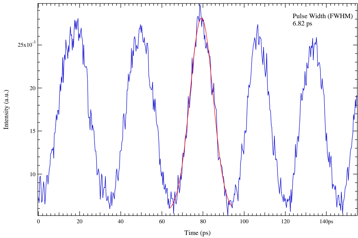
Figure 3-25 Pulse width associated with the sixth harmonic repetition rate
