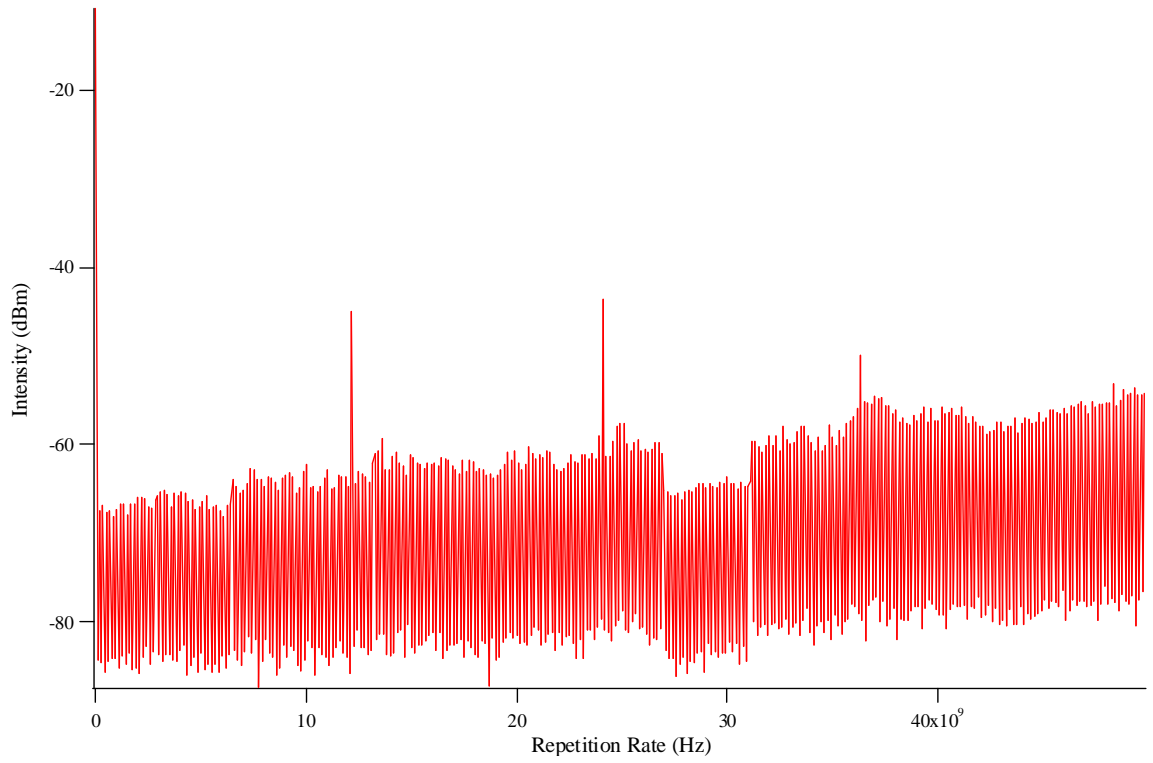
Figure 3-8 50 GHz span of repetition rate while configured for second harmonic generation
