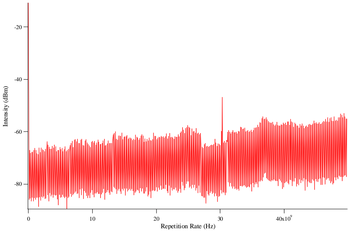
Figure 3-18 50 GHz span of repetition rate while configured for fifth harmonic generation
