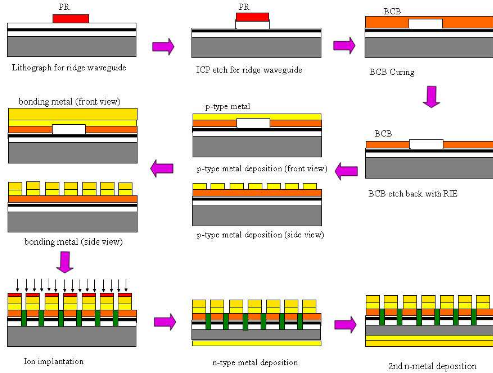
Figure 2-6 Standard processing for standard segmented contact devices [32]
