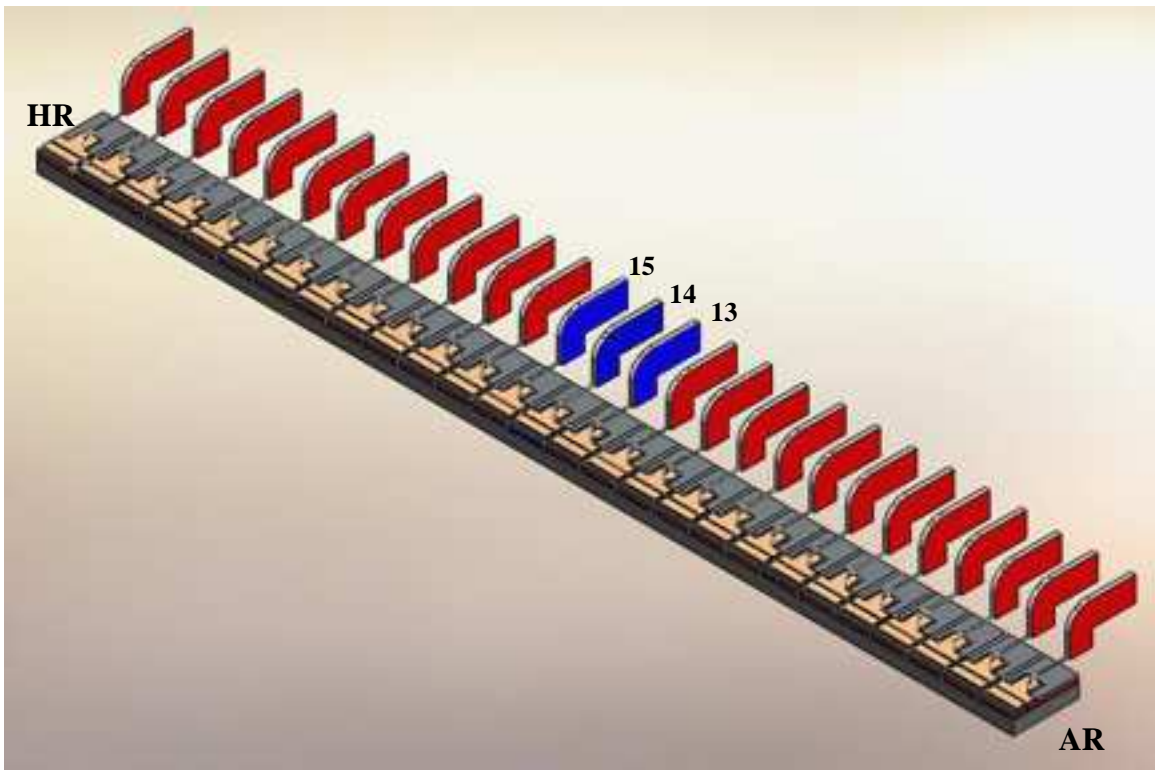
Figure 3-5 Configuration for the generation of the second harmonic using three saturable absorbers
