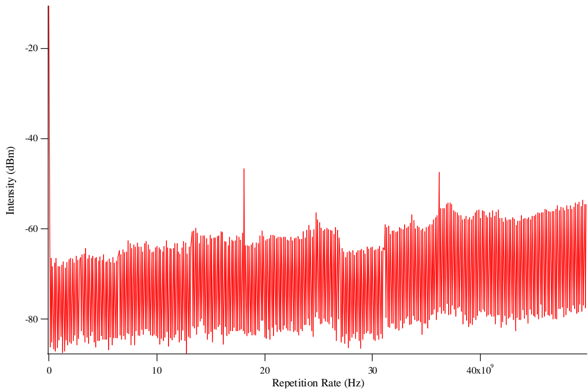
Figure 3-13 50 GHz span of repetition rate while configured for third harmonic generation
