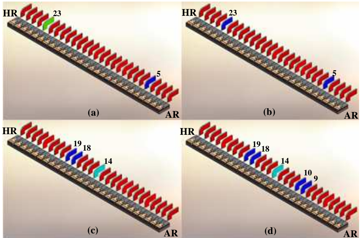
Figure 3-21 Possible configuration for the generation of the sixth harmonic. (a) Using the traditional method and placing a saturable absorber at either section 5 or 23, (b) using both sections 5 and 23, (c) using the double-interval technique by placing saturable absorbers at section 14 and 18&19, and (d) using the double-interval technique by placing saturable absorbers at section 14 and 9&10 and 18&19
