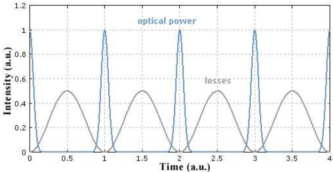
Figure 1-2 Generation of optical pulses by active mode-locking [11]
